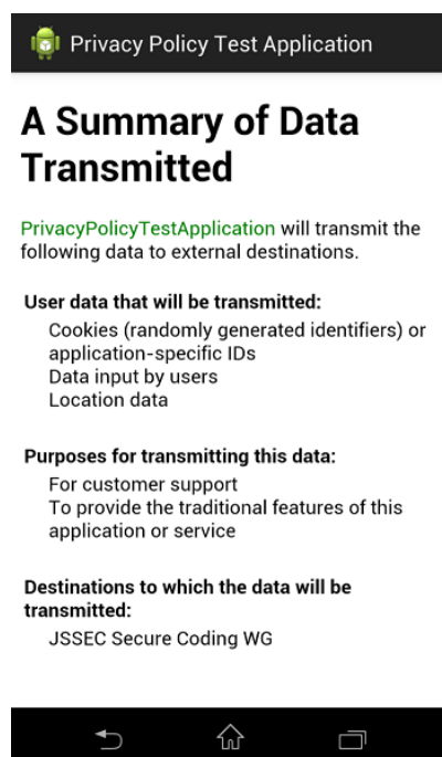
Fig. 5.5.1: Sample of Abstract Application Privacy Policy
