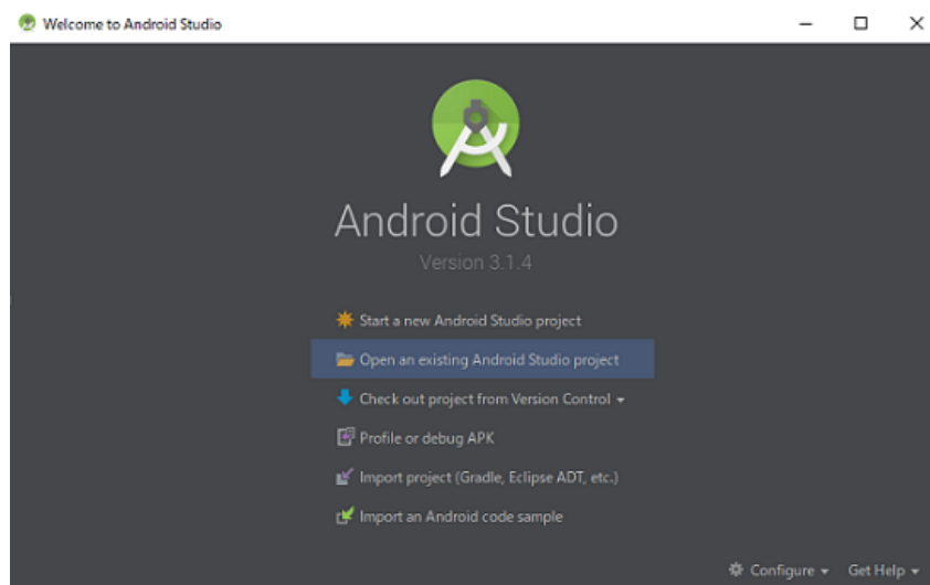
Fig. 2.5.7: Open Project
