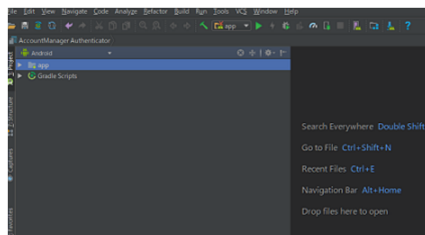
Fig. 2.5.12: Finish Opening
