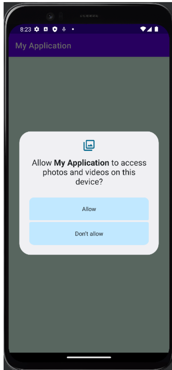
Fig. 4.6.1: READ_MEDIA_IMAGES
