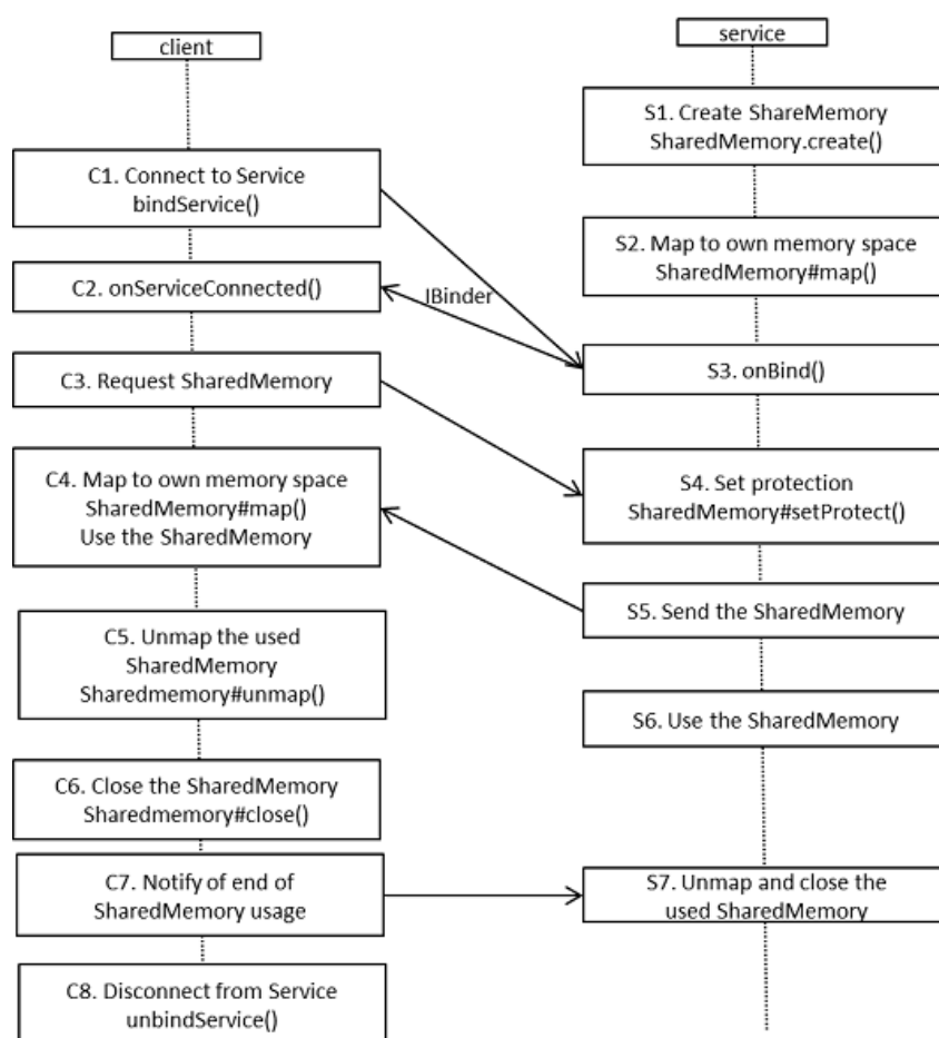
Fig. 4.11.2: Exchanges between shared memory service and client
